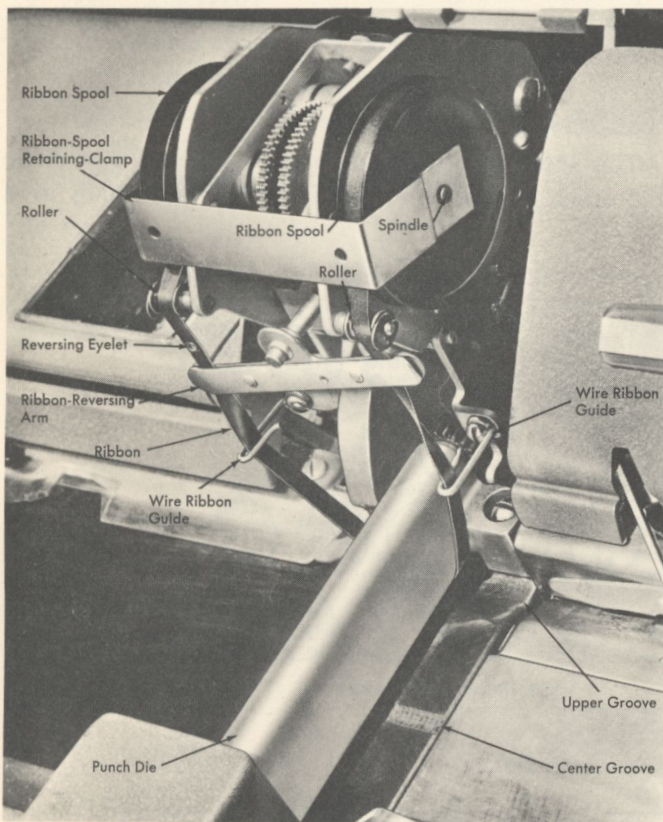
Figure 27. Ribbon Replacement
