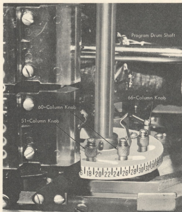
Figure 22. Program Cam Extension Knobs (80-Column Card Setting)
