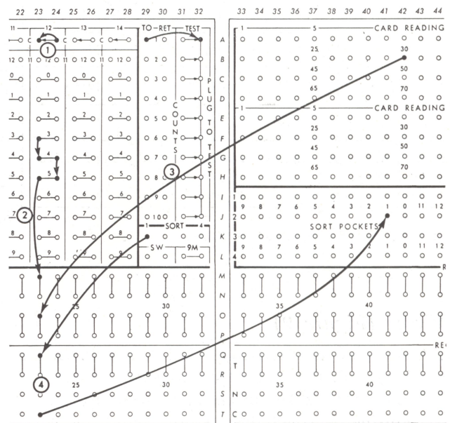
Figure 12. Digit Emitter Method
