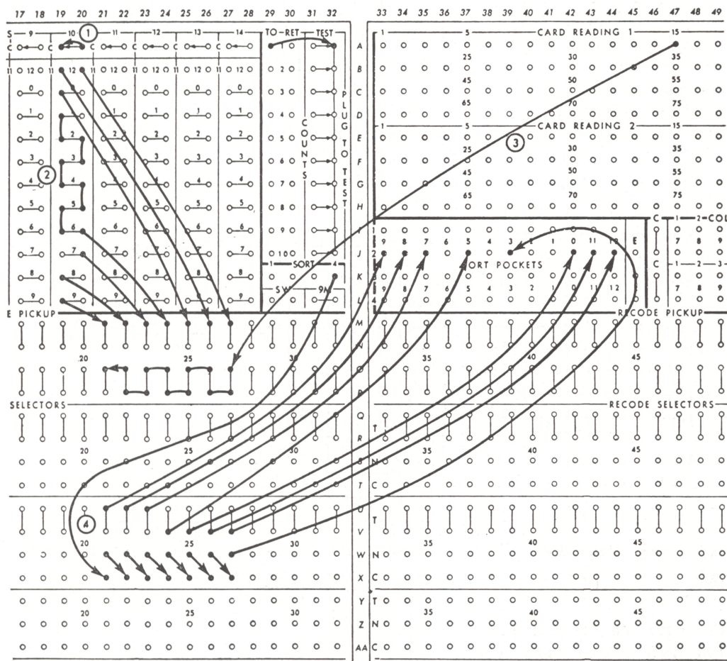
Figure 13. Sorting Cards into Various Pockets Using Recode Selectors
