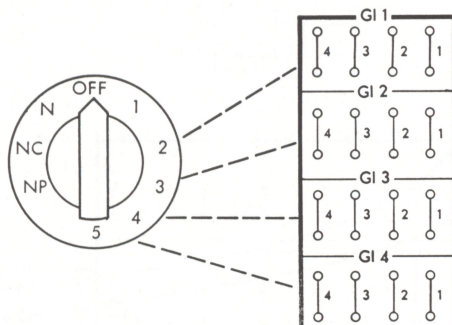
Wiring (Figure 24)
