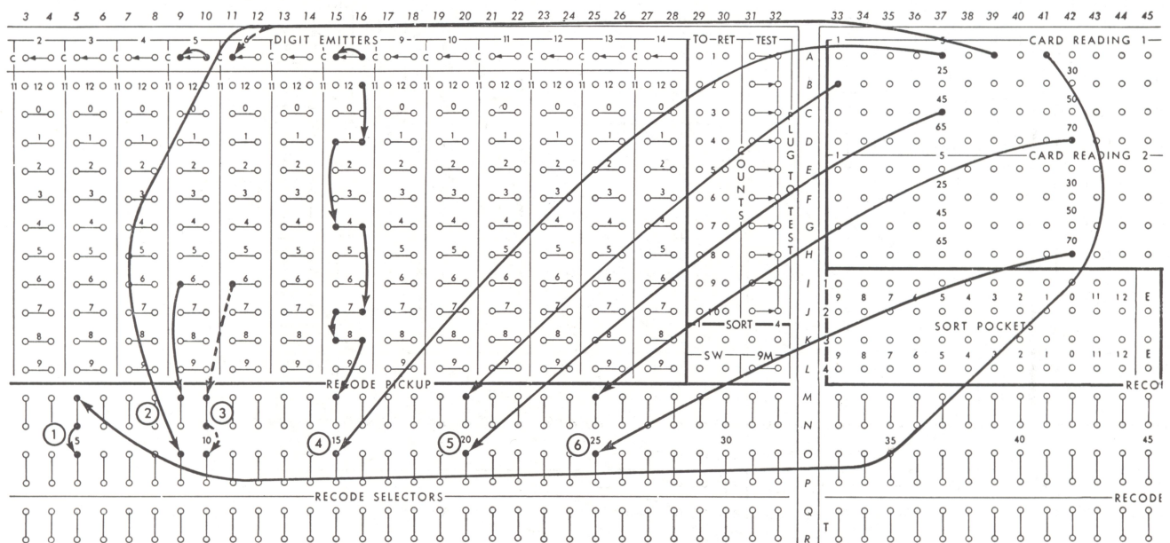
Figure 14. Recode Selector Pickup
