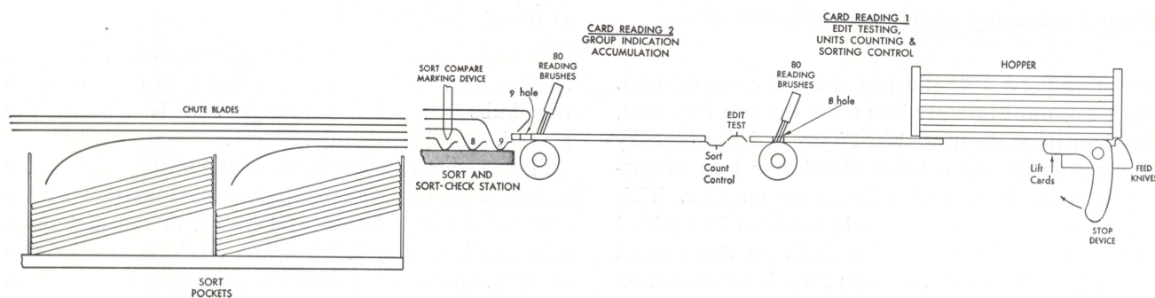
Figure 3. Path of Cards through the Machine
