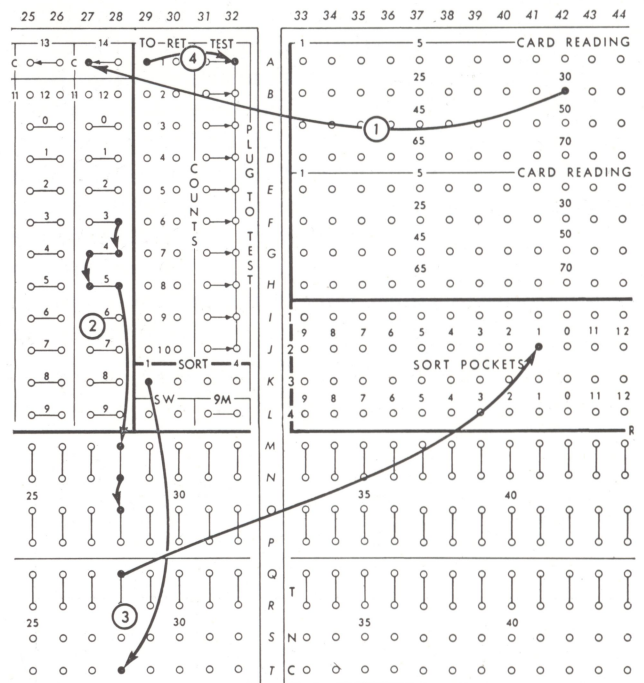
Figure 11. Digit Selector Method
