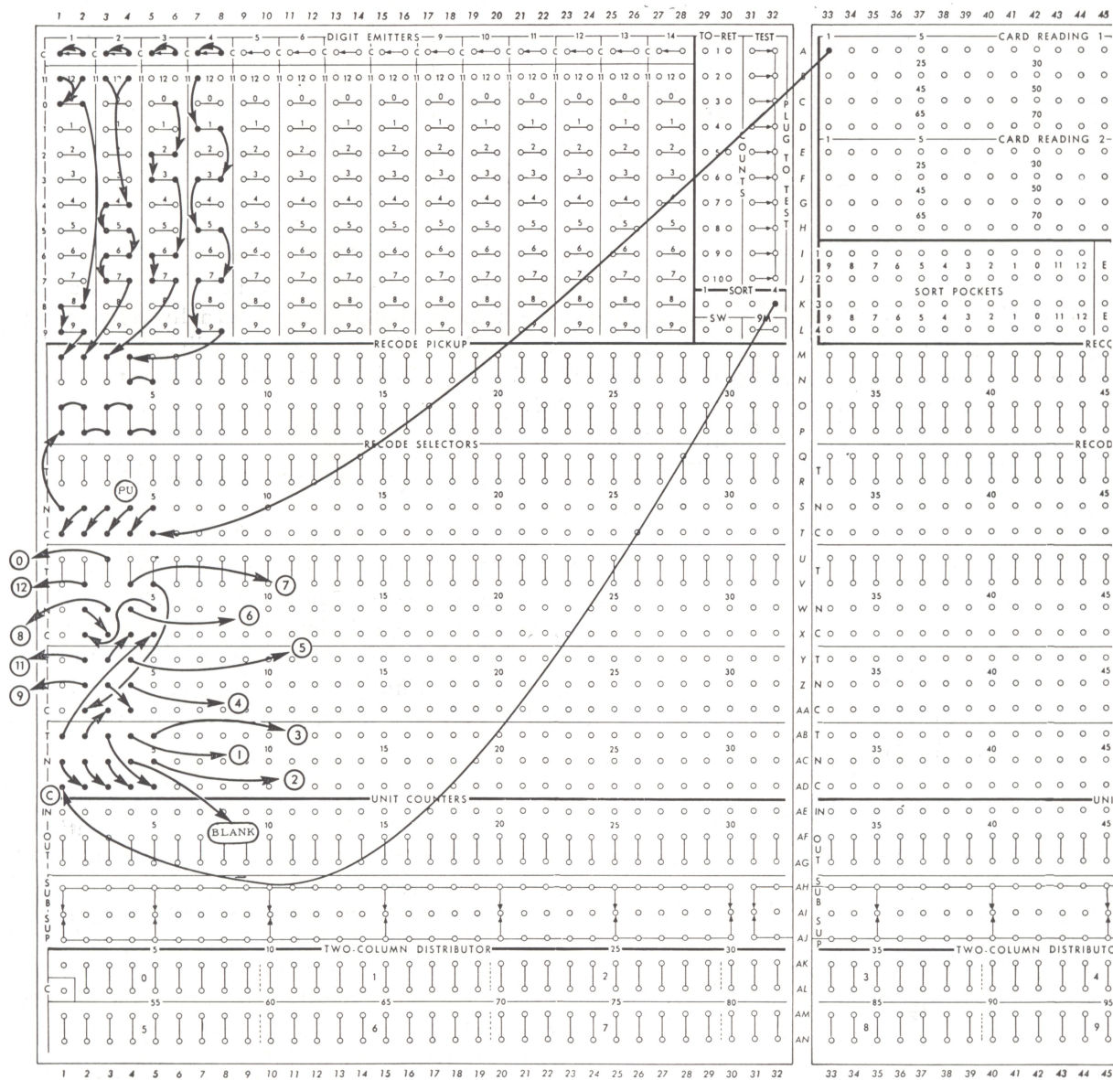
Figure 62. Five Recode Selectors as a Substitute for a Column Distributor
