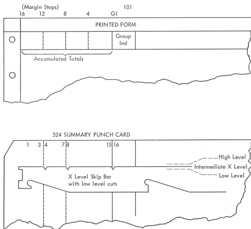
Figure 33. Margin Stop and Skip Bar
