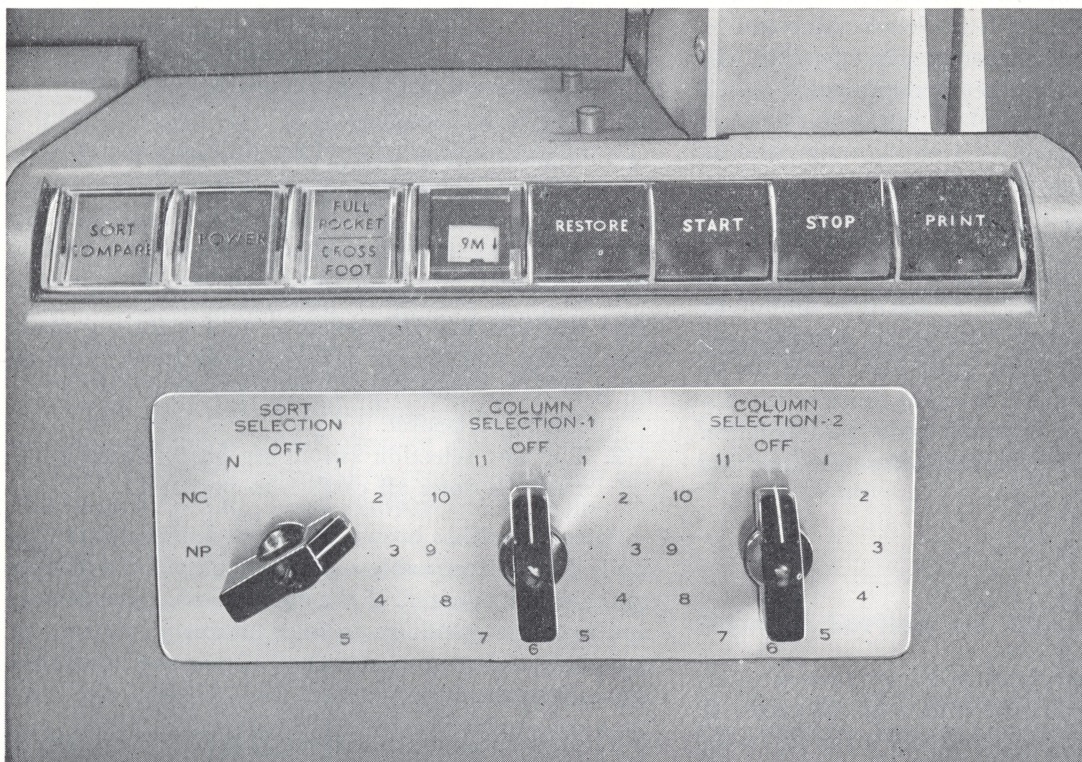
Figure 1. Lights, Keys, and Switches
