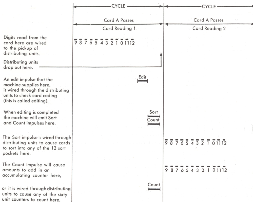
Figure 6. Schematic of Machine Operation
