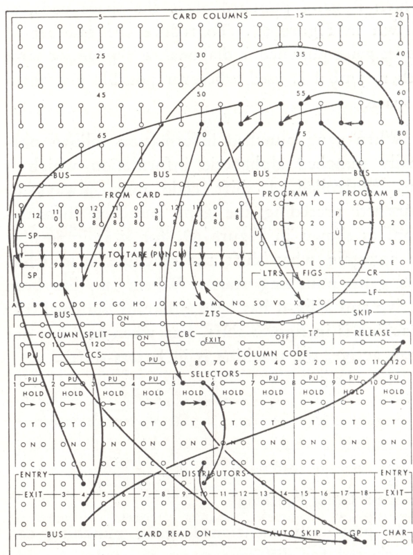
FIGURE 68. WIRING FOR FIGURE 67
