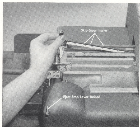
FIGURE 10. INSERTING THE ADJUSTABLE SKIP BAR
