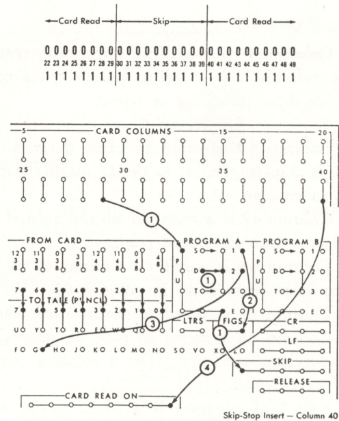
FIGURE 23. PROGRAM PUNCHING A FIG-G AFTER A LETTER OR SPACE
