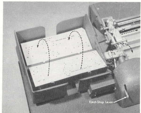
FIGURE 6. CARD REVERSING DEVICE
