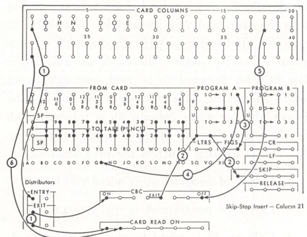
FIGURE 46. CBC CONTROLS PROGRAM PUNCHING AND SKIPPING
