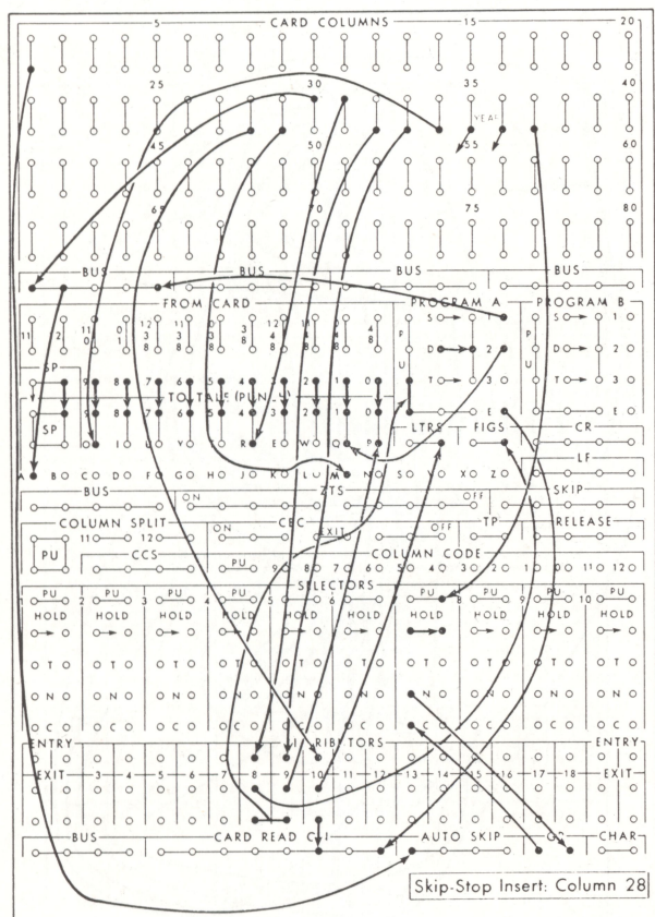
FIGURE 66. WIRING FOR FIGURE 65
