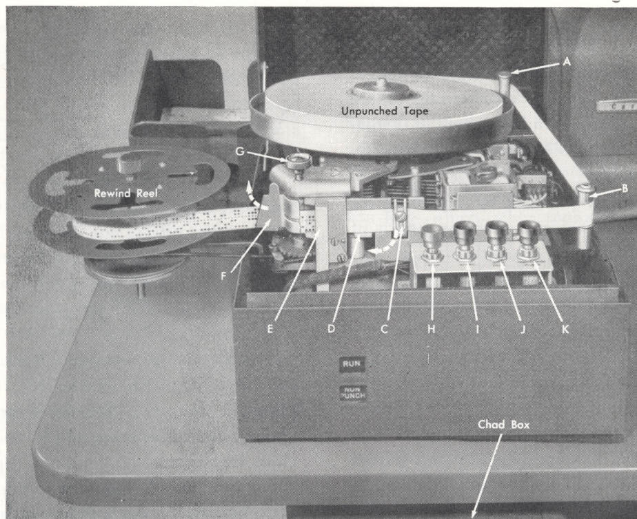
FIGURE 11. TAPE PUNCHING UNIT WITH COVER RAISED FOR TAPE THREADING
