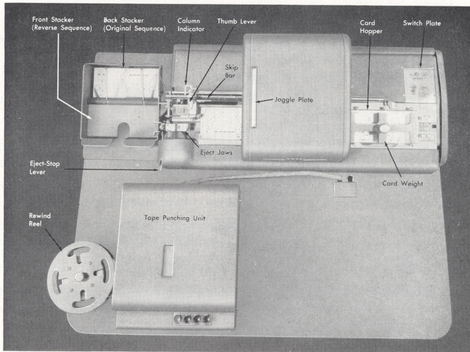
FIGURE 5. MACHINE FEATURES
