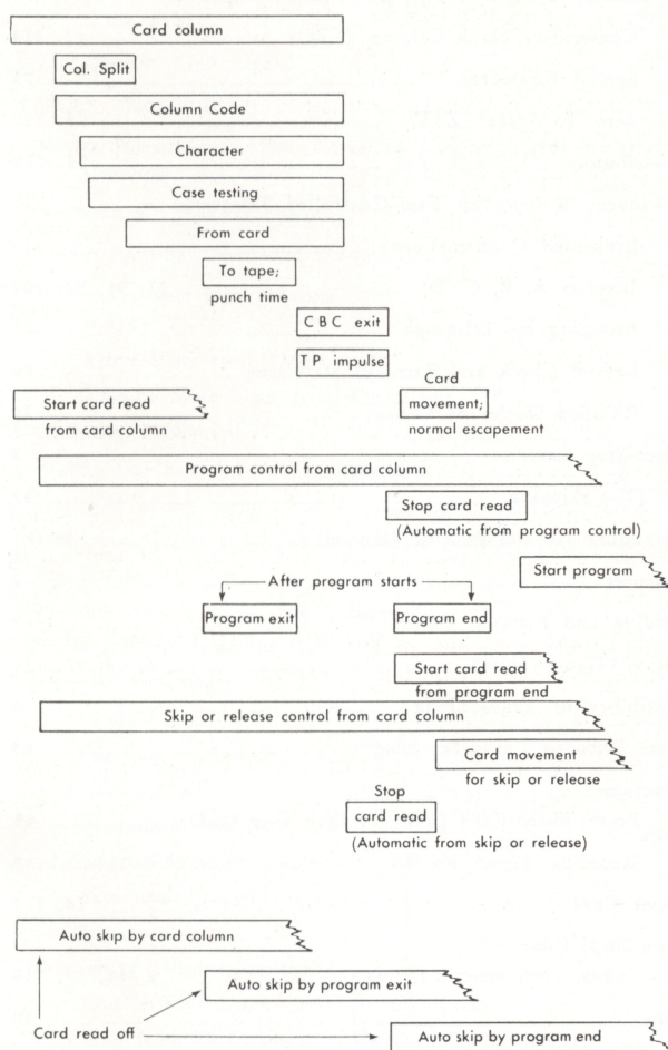
FIGURE 111. SEQUENCE, DURATION, AND RELATIONSHIP OF ALL IMPULSES
