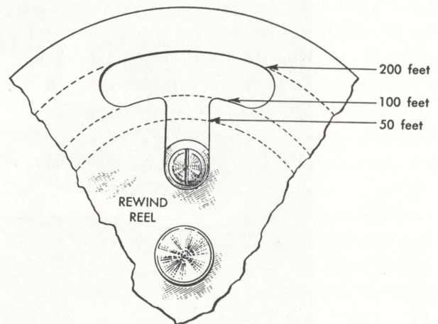
FIGURE 12. GAUGING THE TAPE LENGTH
