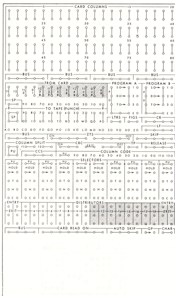
FIGURE 13. CONTROL PANEL
