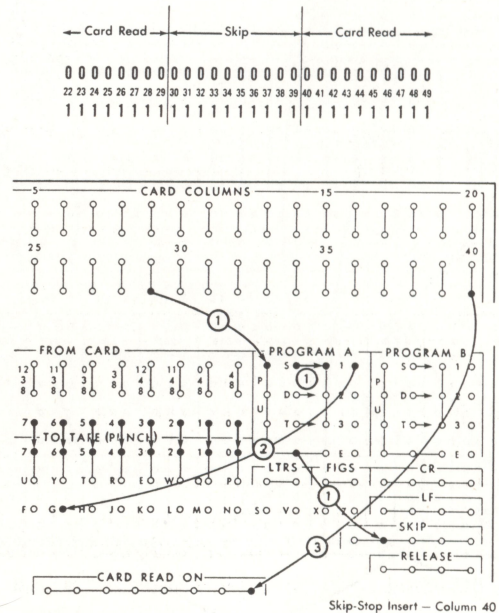
FIGURE 24. PROGRAM PUNCHING A FIG-G AFTER A NUMERAL
