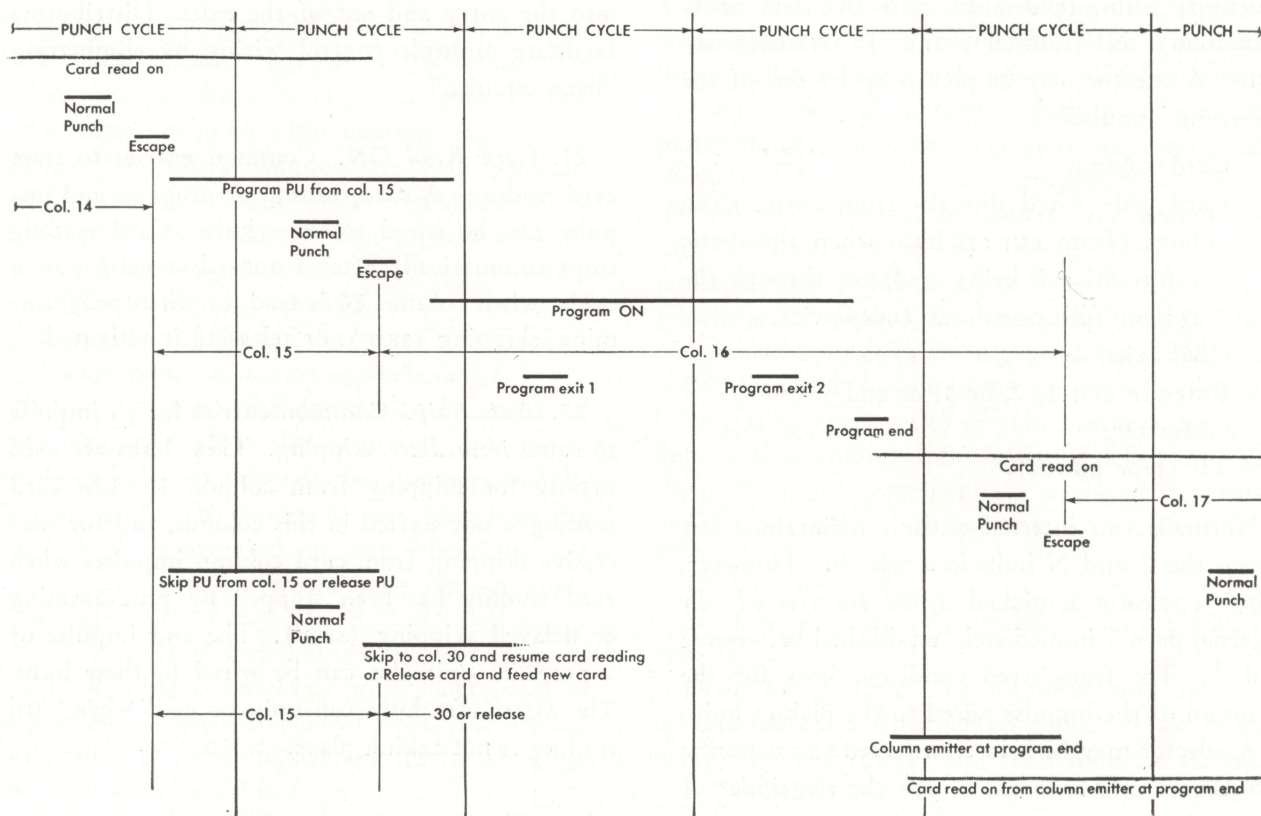
FIGURE 110. SEQUENCE OF PROGRAM PUNCHING
